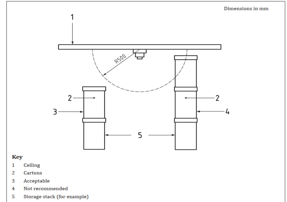
Figure 13 — Clear space around a detector [see 22.3p]]
